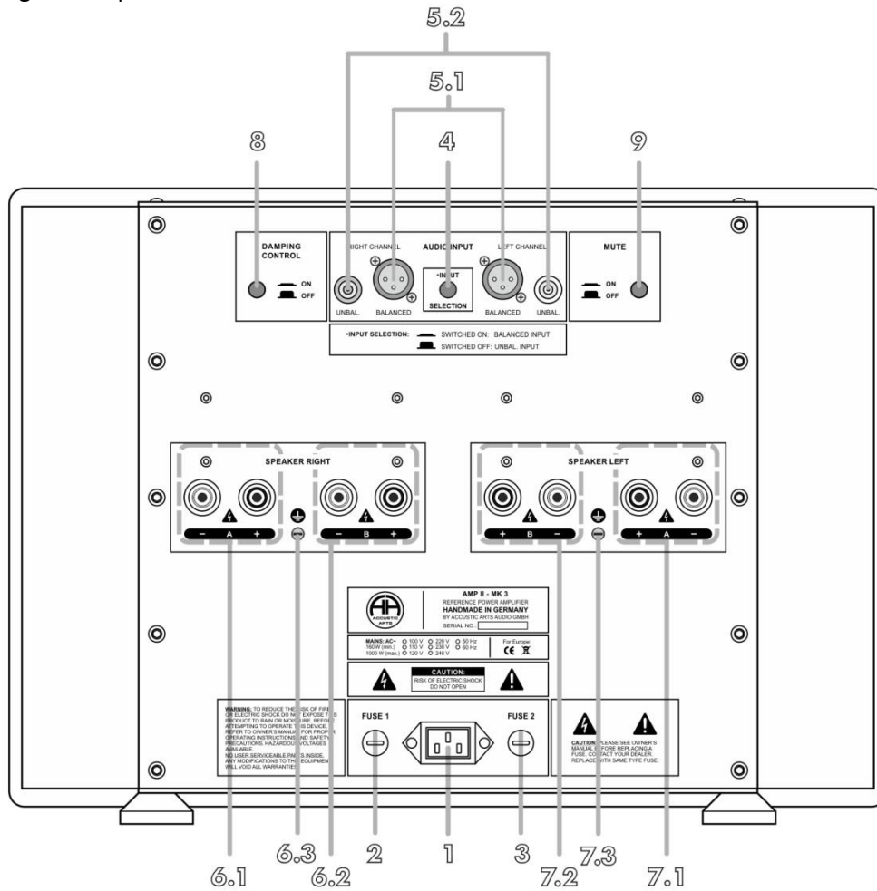
Fig. 1: Rear panel
