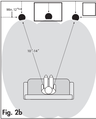
MC6-HT: Front left, center, and right speakers.
