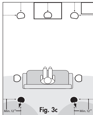
MC6-HT: Non-direct rear channels in a 7.1-channel system.
