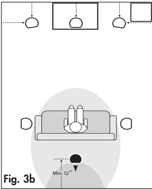
MC6-HT: Non-direct rear channel in a 6.1-channel system.
