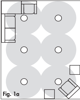
MC4/6/8: Multiple speakers, distributed audio.
